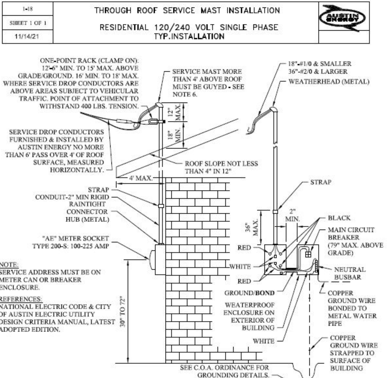
Figure 1-18. Through-Roof Service Mast Installation (Residential – Typical Overhead Installation)
